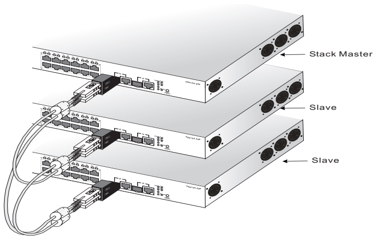
Figure 3-7. Connecting Switches in a Stack
